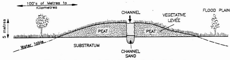
Fig. . Schematic cross-section through an active low sinuosity channel.
