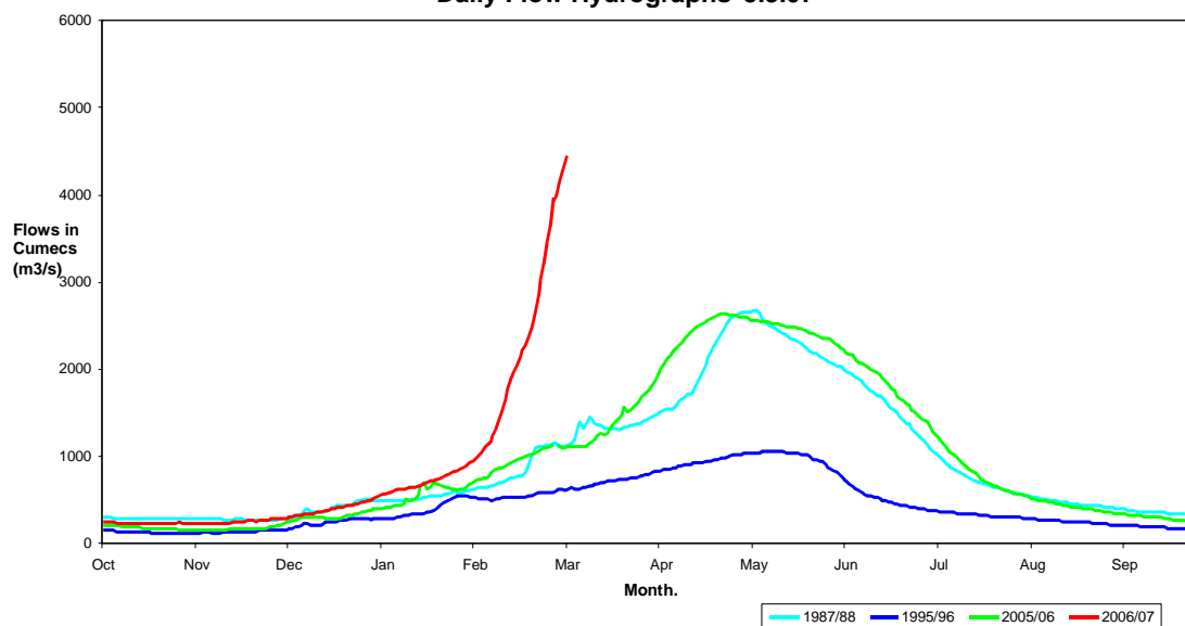
Figure 2 - Zambezi River At Vic Falls. Daily Flow Hydrographs 5.3.07
